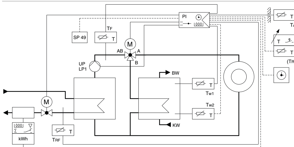
Weather-dependent supply-temperature control (secondary) in converter systems with drinking water priority switching via diverting valve.
