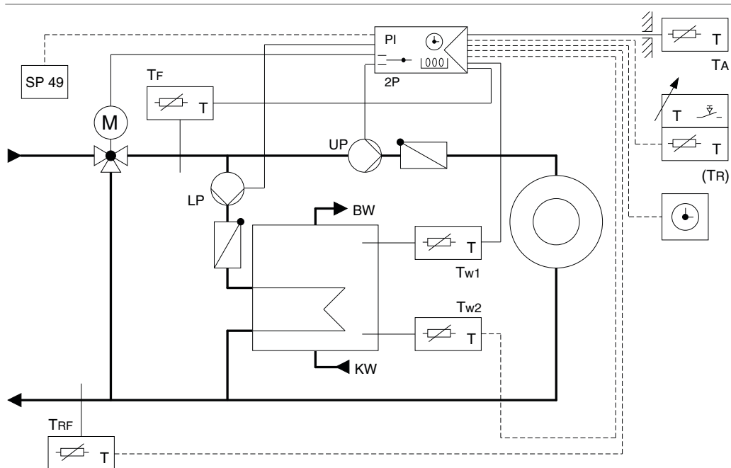
Weather-dependent supply-temperature control and drinking-water control via control valve.
