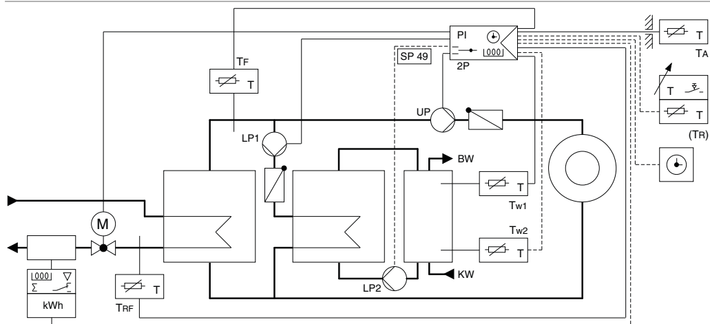
Weather-dependent supply-temperature control (secondary) in converter systems with drinking-water control by means of 2 charge pumps via additional converters (charger system).
