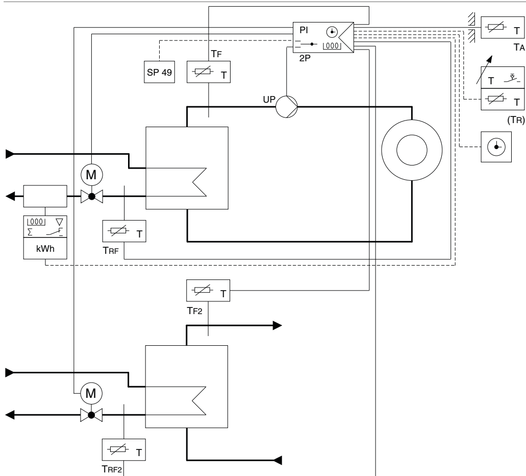
Weather-dependent supply-temperature control (secondary) and separate fixed-value control (secondary) for drinking water circuit in converter systems.
