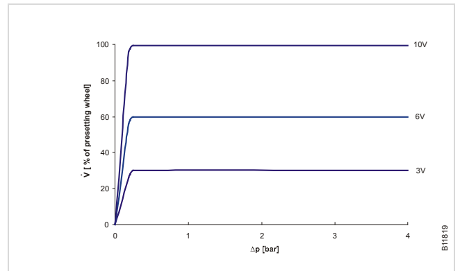
Example function: DN 40 VCL040F200 with preset max. volume flow 7500 l/h Volume flow as a function of the control voltage (0...10 V continuous control) and the differential pressure Control voltage: 3 V, 6 V and 10 V
